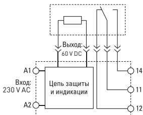
PM Slim 23/1 230VAC/60VDC EKF AVERES
