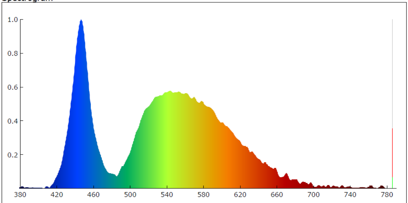
Spectrogram
